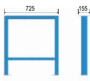
Legs
