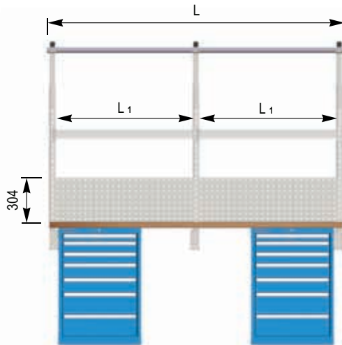
Length 2000 / 2500 / 3000 mm
