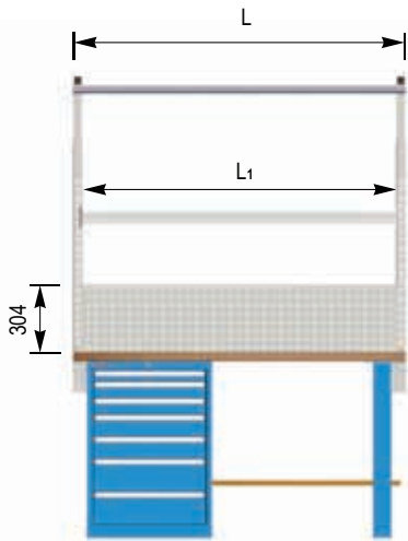
Length 1250 / 1500 / 1750 mm
